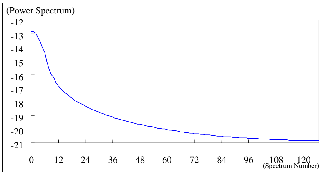
(Figure 30) Fourier Transformation
