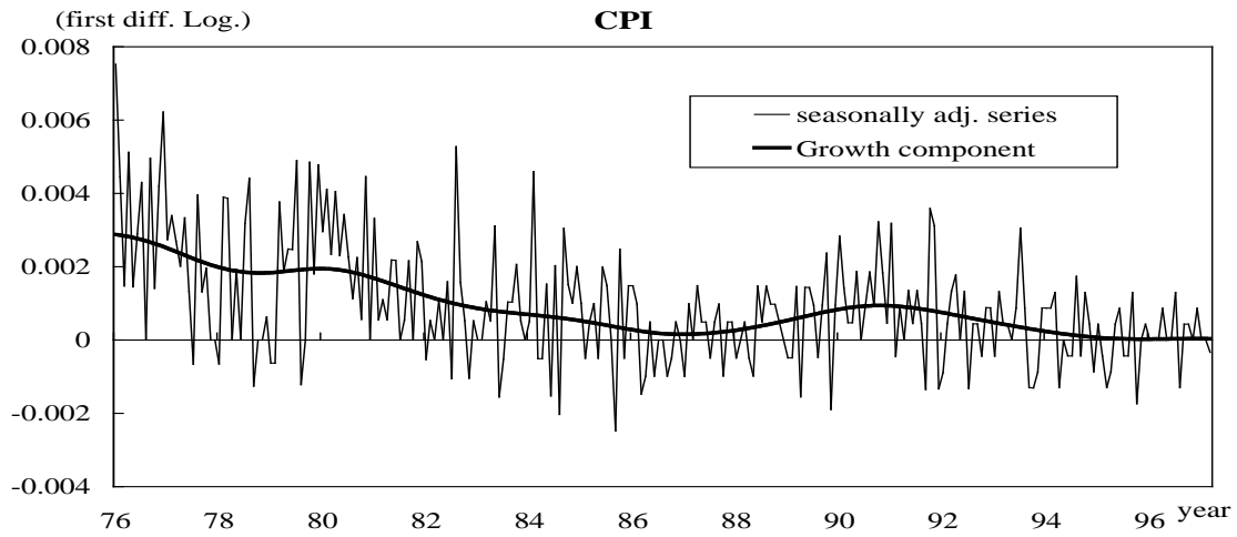
(Figure 15) Growth (trend-cycle) components extracted by HP filter ( \lambda = 14400 )
