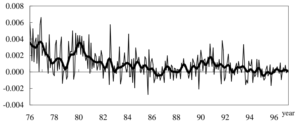
(2) Moving Average: 13 terms
