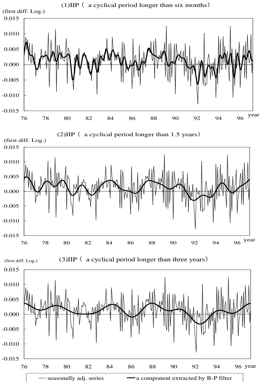
(Figure 13-3) Trend-cycle components of IIP extracted by Band-Pass filter
