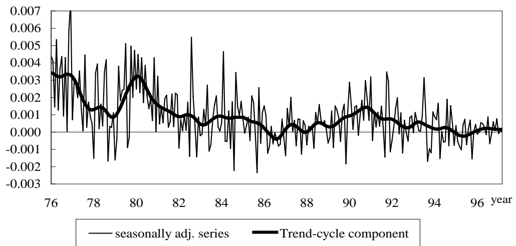
(3) Moving Average: 23 terms
