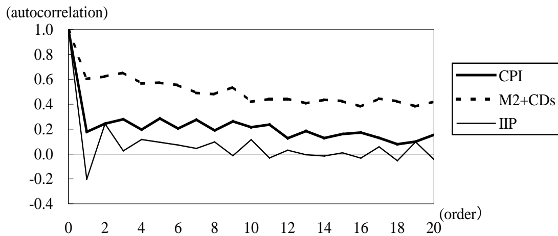
(Figure 5) Autocorrelation of each time series (first difference in logarithm, seasonally adjusted)
