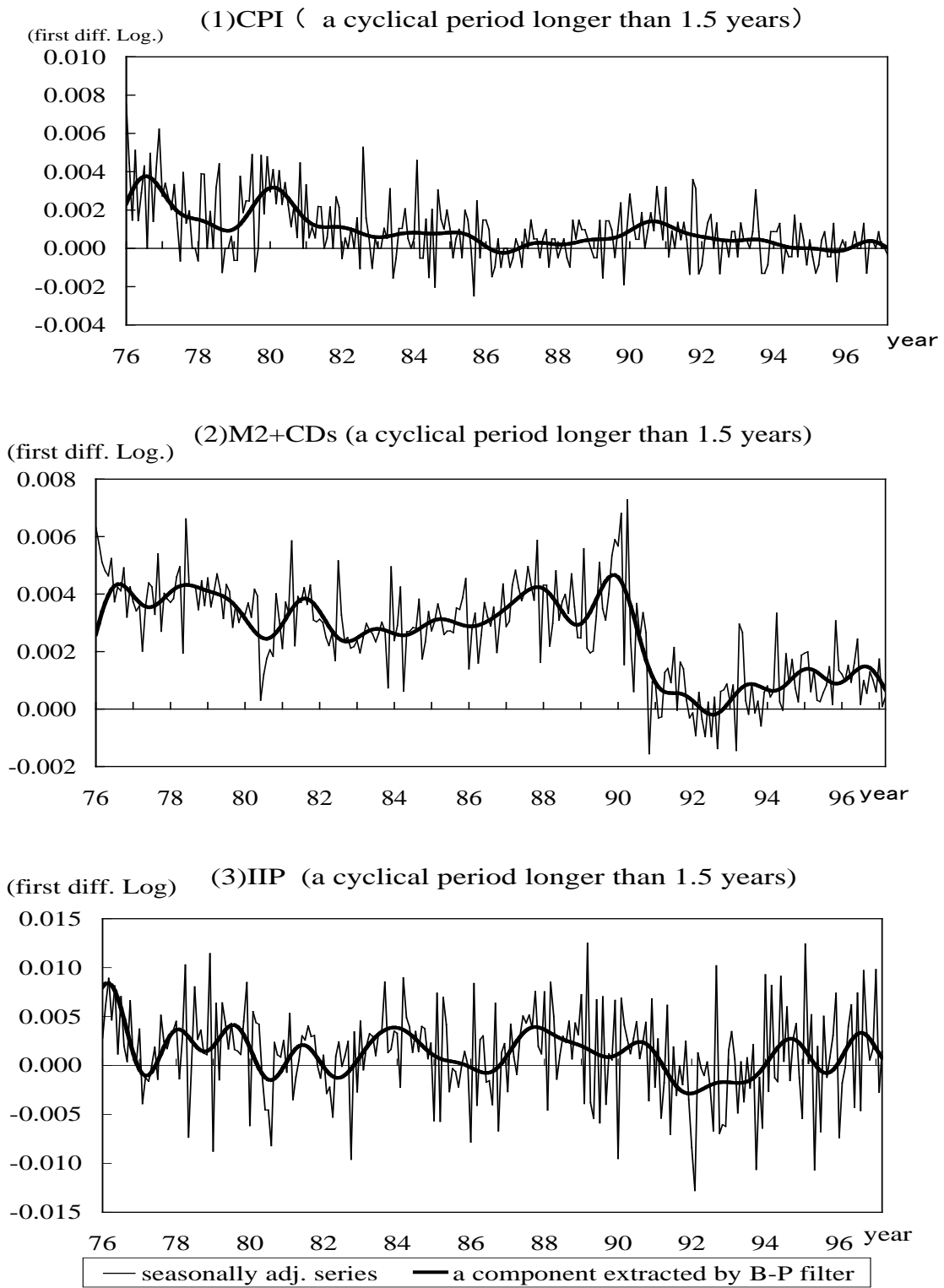
(Figure 14) Trend-cycle components extracted by Band-Pass filter (with one year out-of-sample forecast by ARIMA)
