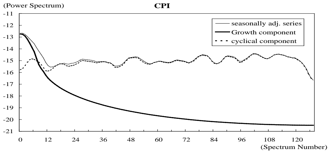
(Figure 16) The Power Spectra of components extracted by HP filter
