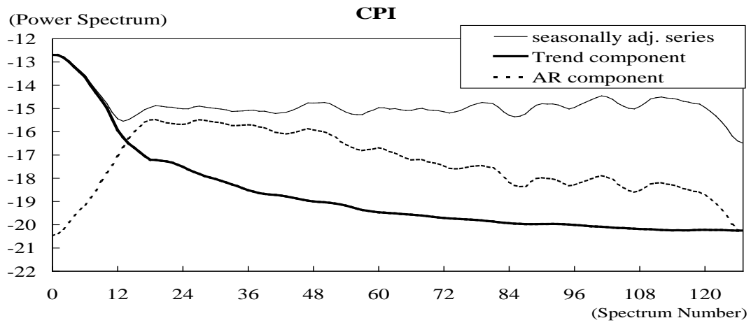
(Figure 19) The Power Spectra of components extracted by DECOMP
