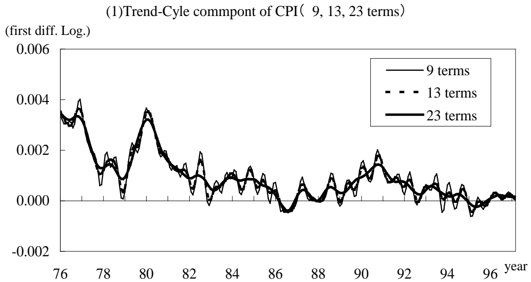
(Figure 9) Trend-cycle components of CPI extracted by Henderson Moving Average: differences by terms
