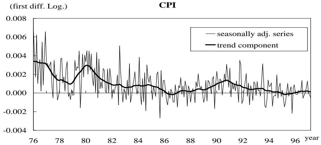
(Figure 18) Trend (trend-cycle) components extracted by DECOMP
