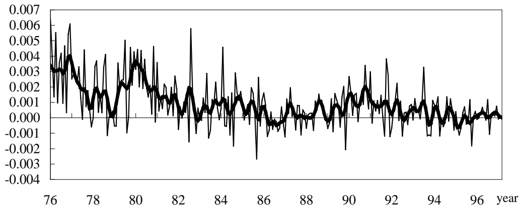
(1) Moving Average: 9 terms
