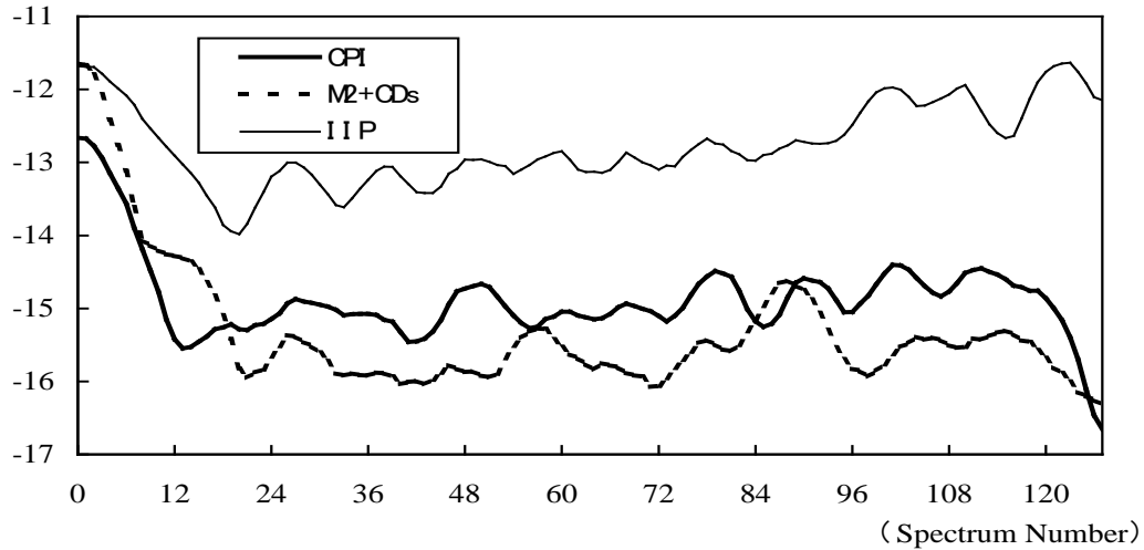
(Figure 6) The Power Spectra of each time series (first difference in logarithm, seasonally adjusted. Power Spectrum (natural logarithm))
