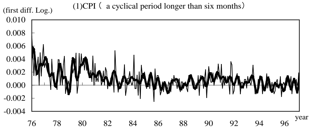
(Figure 13-1) Trend-cycle components of CPI extracted by Band-Pass filter (first difference in logarithm)
