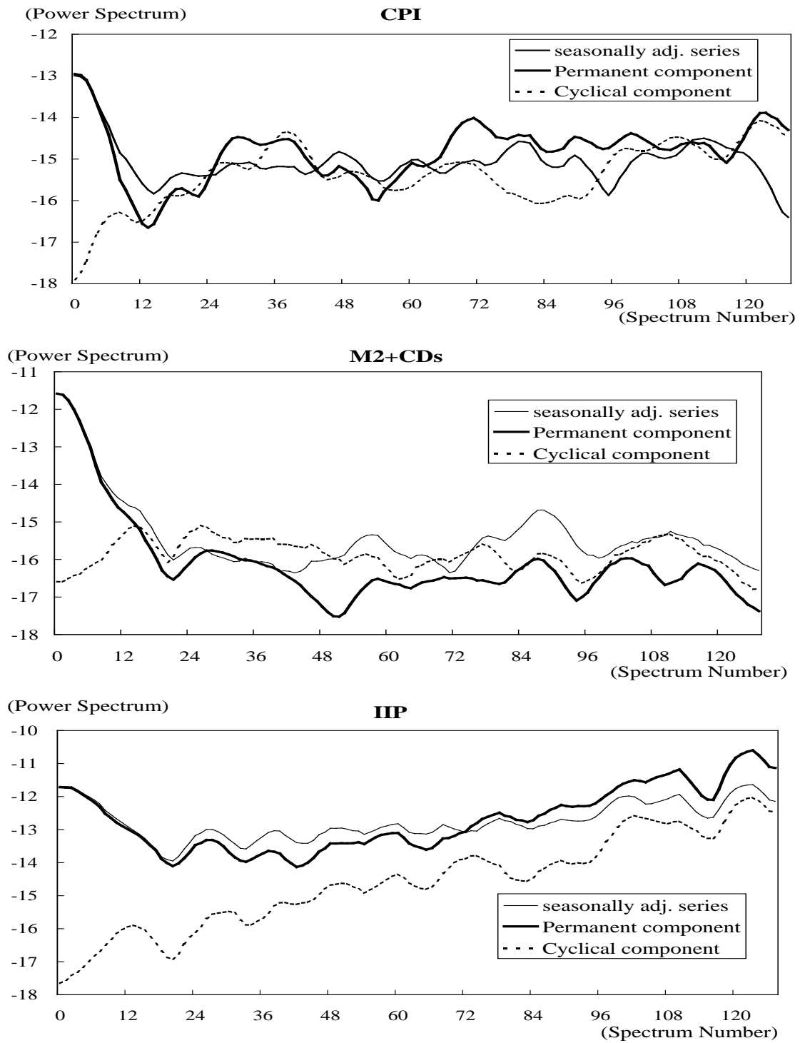
(Figure 21) The Power Spectra of components extracted by Beveridge and Nelson method
