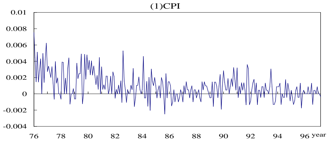
(Figure 2) The graphical movements of each time series (first difference in logarithm, seasonally adjusted)
