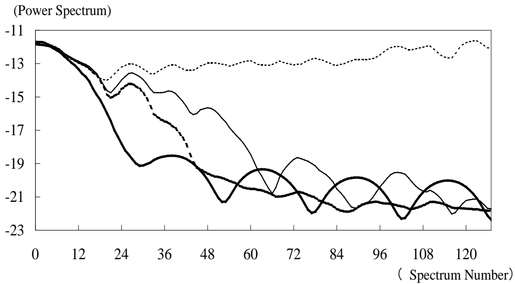
(2) Power Spectra of Trend-cycle components (IIP)
