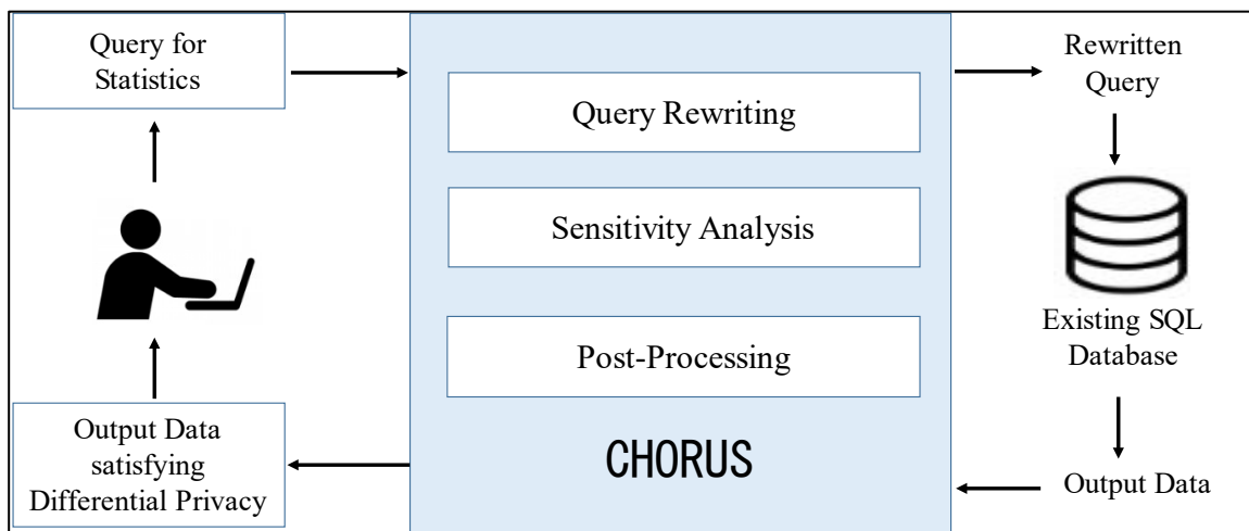
Figure 4 Overview of CHORUS
