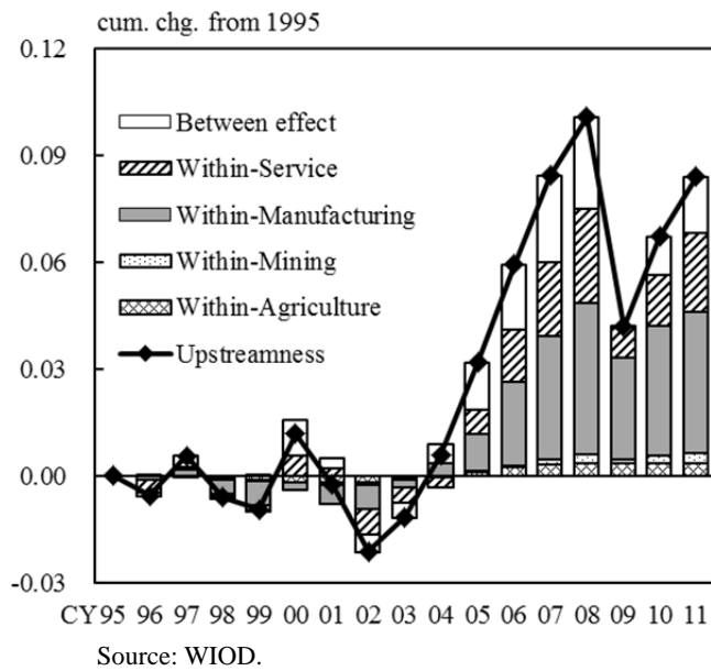
Figure 1: Global upstreamness (1995–2011)
