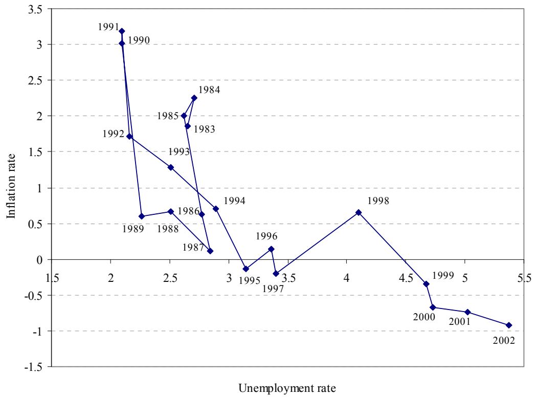
Figure 1: Inflation/Unemployment Plot, 1983-2002
