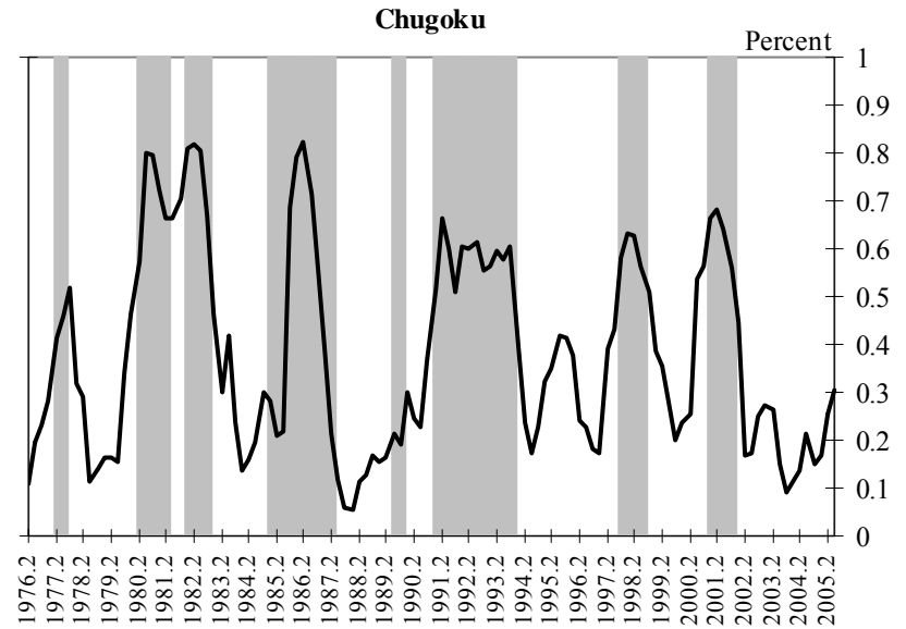
Figure 6 (continued) Regional Recession Probabilities (Shaded areas are national IIP recessions)
