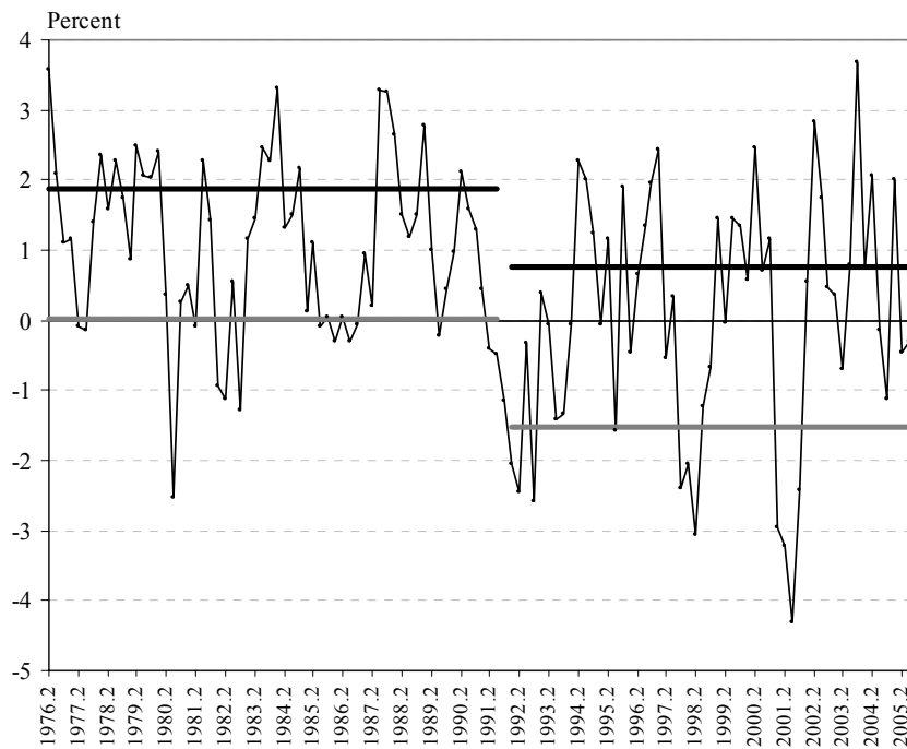
Figure 3 Growth of IIP: Japan, With Structural Break (Thick black line is expansion growth rate, thick gray line is recession growth rate)
