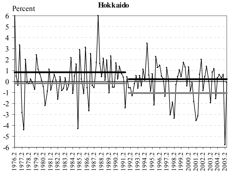
Figure 5 Actual and Average IIP Growth Rates: Regions, With Structural Break (Thick black lines are average expansion growth rates, thick gray lines are average recession growth rates)
