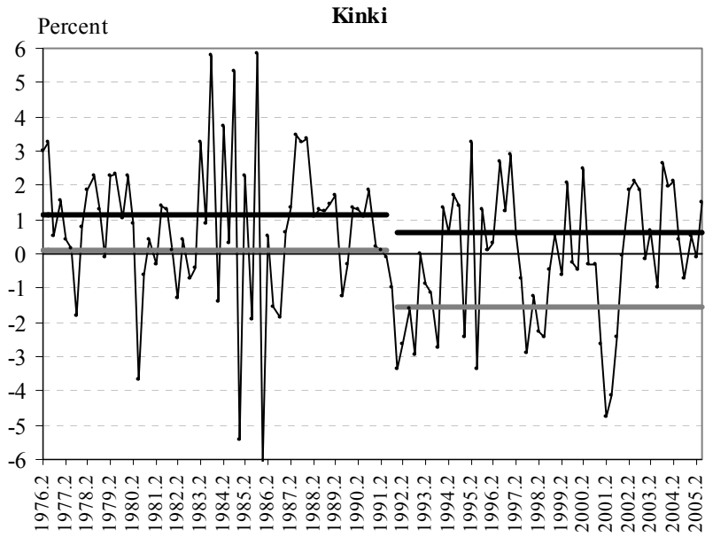
Figure 5 (continued) Actual and Average IIP Growth Rates: Regions, With Structural Break (Thick black lines are average expansion growth rates, thick gray lines are average recession growth rates)
