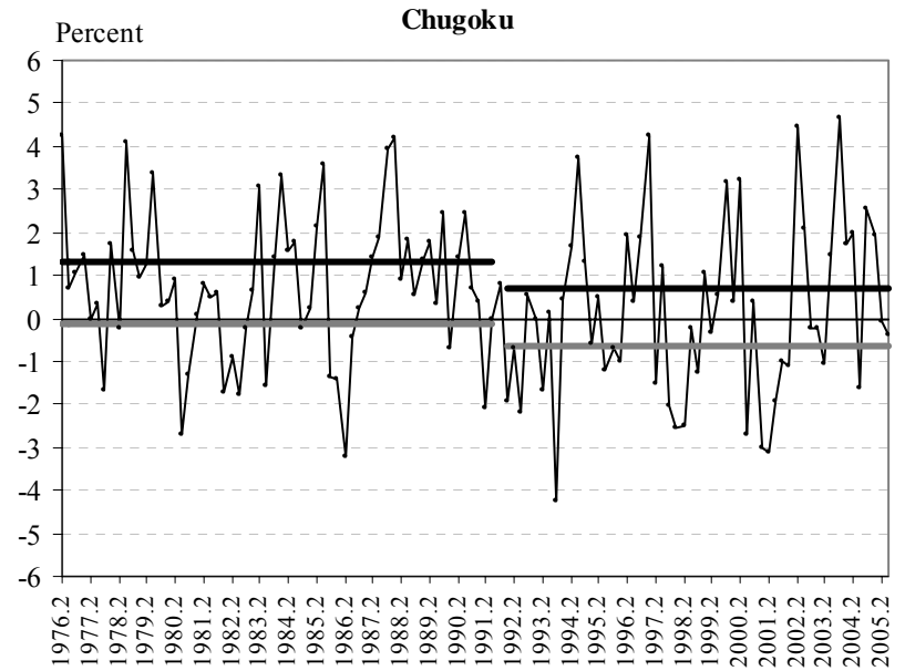
Figure 5 (continued) Actual and Average IIP Growth Rates: Regions, With Structural Break (Thick black lines are average expansion growth rates, thick gray lines are average recession growth rates)
