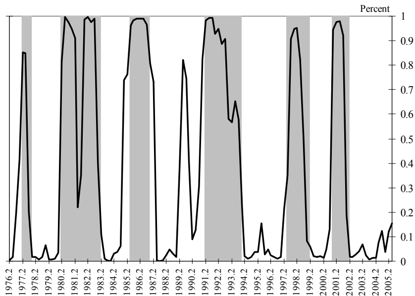
Figure 4 Probability of Japanese Recession, With Structural Break (Shaded area are ESRI recessions)
