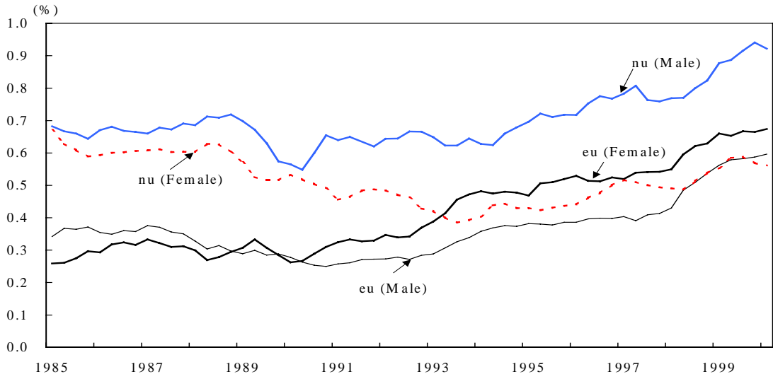
Figure 4: Transition Probabilities
