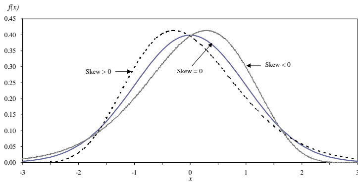
Figure 1. Skewness
