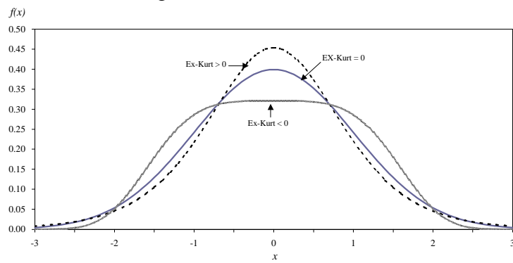
Figure 2. Excess Kurtosis
