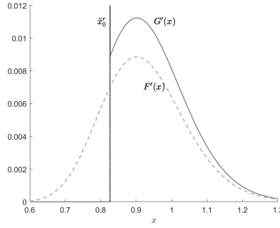
Figure 3: Distribution for F'(x) and G'(x)
